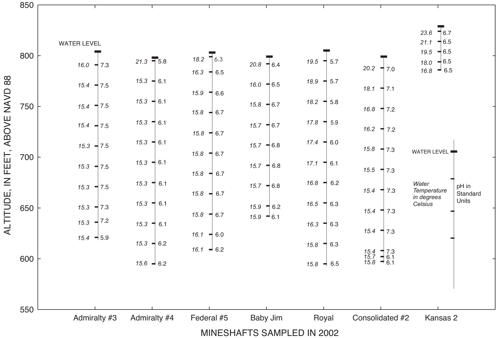
Figure 2. Water levels, pH, and temperature of water at selected depths in mineshafts sampled in 2002, Picher mining district.
