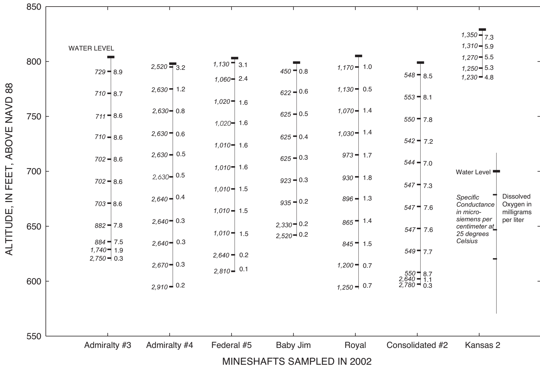
Figure 3. Water levels, specific conductance, and dissolved oxygen of water at selected depths in mineshafts sampled in 2002, Picher mining district.
